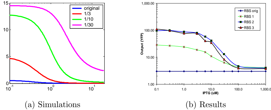
Figure 13. Simulations and experimental results demonstrating the effect of modifying RBS efficiencies on circuit performance.
