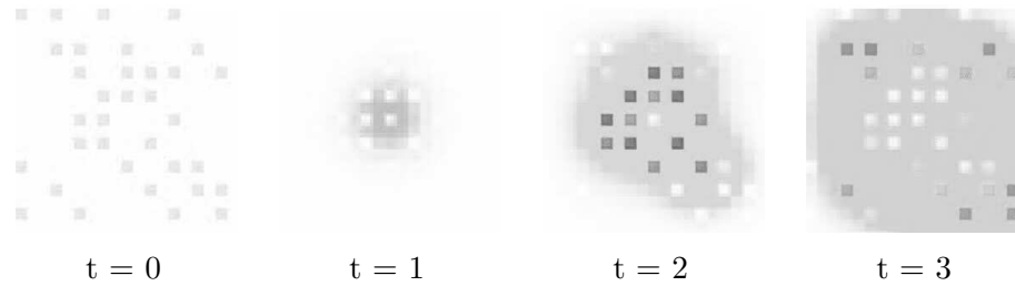
Figure 27. Simulation of the band detect circuit with a sender cell in the center, 35 receiver cells, and diffusion of 3OC_6HSL .
