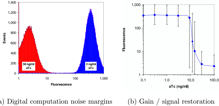
Figure 12. Transfer curve gain and noise margins for the lacI/p(lac) circuit.
