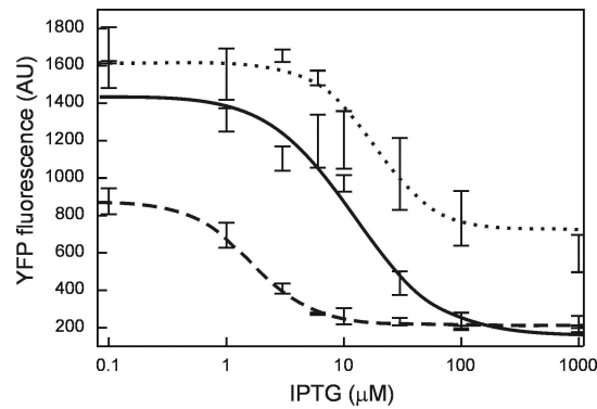
Figure 15. Experimental results demonstrating the ability to optimize system response using directed evolution. Curves are best fit to data points using a standard Hill equations, and error bars represent the results of triplicate experiments.
